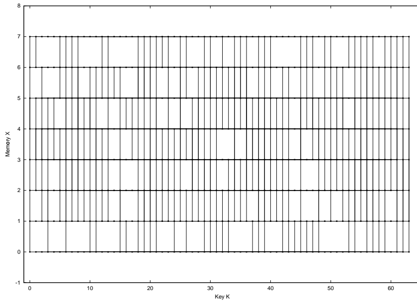
Fig. 4. Grid-contour of a \mathcal{R} -maximizing mapping: scenario (S_1) .
